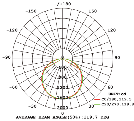
Polar Curve
