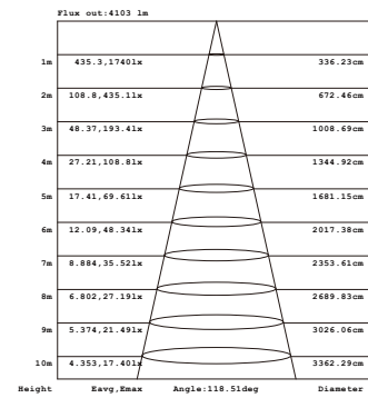
Cone Chart
